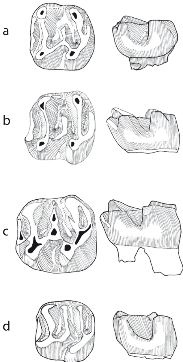
Text-fig. 7. Comparison of lower molars of different Eomyidae in occlusal (left) and labial (right) view. a) Eomys helveticus n. sp. from Rigi 1, M_{1/2} sin.: Rgi 3, holotype. b) Eomys schluengeri n. sp. from Rigi 2, M_1 dext. (reversed): Rgi 20, holotype. c) Eomys molassicus ENGESSER, 1987 from Rigi 2, M_1 sin.: DKR-gi13. d) Eomyodon mayoi ENGESSER, 1990 from Krummenau/Thur, M_1 dext. (reversed): Tpl A16. All figures at magnification 35 \times .
