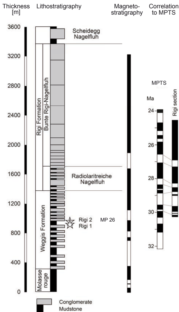
Text-fig. 2. Lithostratigraphy and magnetostratigraphy of the Rigi section with correlation to the MPTS (Magnetopolarity Time Scale) according to Schlunegger (1995). Asterisk = mammal site.
