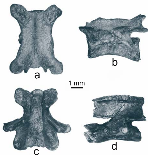
Text-fig. 7. Fossil urodelans from studied localities. a, b – Mioproteus caucasicus , trunk vertebra, dorsal (a) and lateral (b) views; c, d – Chelotriton paradoxus , trunk vertebra, dorsal (c) and lateral (d) view. Scale bar 1 mm.
