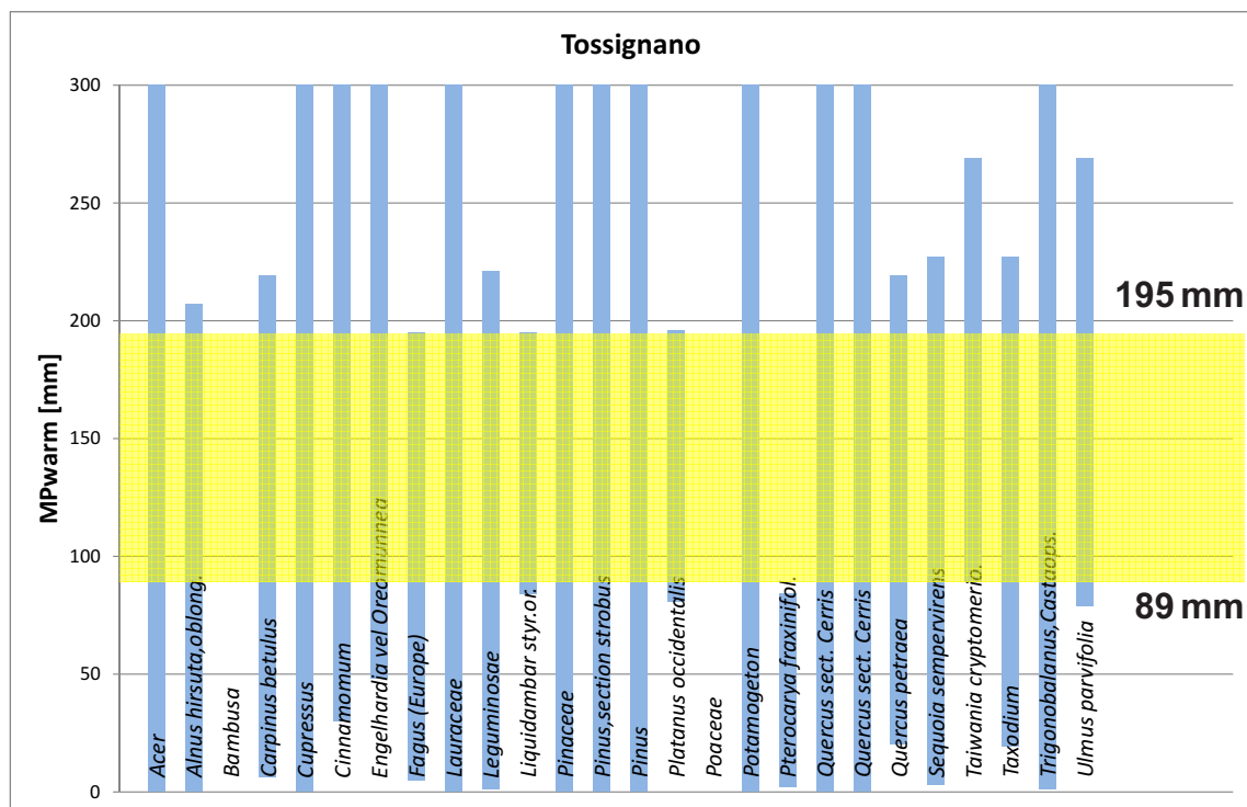
Text-fig. 5. CA climate charts for the Monte Tondo and Tossignano floras, showing climatic ranges of the Nearest Living Relatives of the fossil taxa with respect to MPwarm. For legend see Text-fig. 3.
