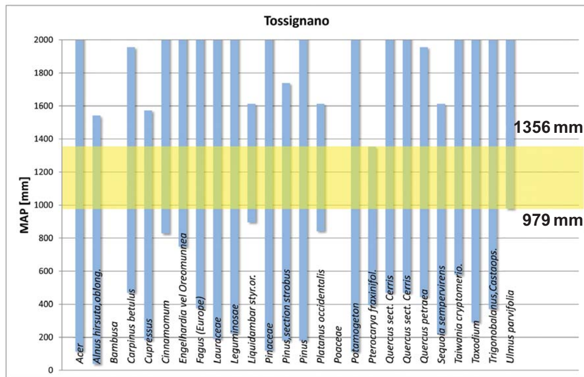
Text-fig. 4. CA climate charts for the Monte Tondo and Tossignano floras, showing climatic ranges of the Nearest Living Relatives of the fossil taxa with respect to MAP. For legend see Text-fig. 3.
