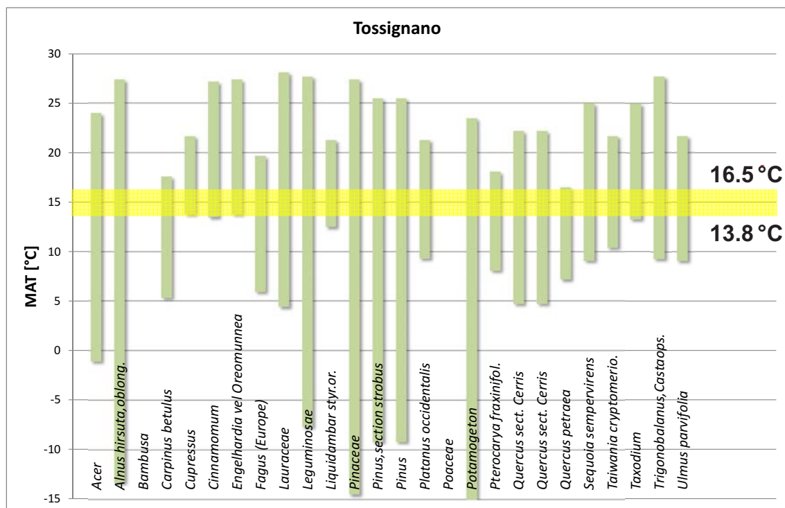
Text-fig. 3. CA climate charts for the Monte Tondo and Tossignano floras, showing climatic ranges of the Nearest Living Relatives of the fossil taxa with respect to MAT. Right-hand positioned large bold figures and shaded areas in each case indicate the Coexistence Interval, with the number of overlapping taxa being at a maximum.
